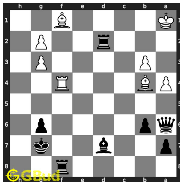
Figure 1: Solve this medium chess puzzle 0104. Mate in 2 moves @ https://gbud.in/gsdm112
