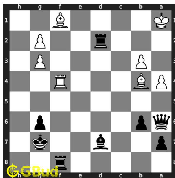
Figure 3: Initial board position of medium chess puzzle 0104
