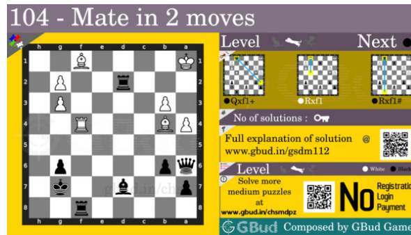
Figure 10: medium chess puzzle 104 chart 4
